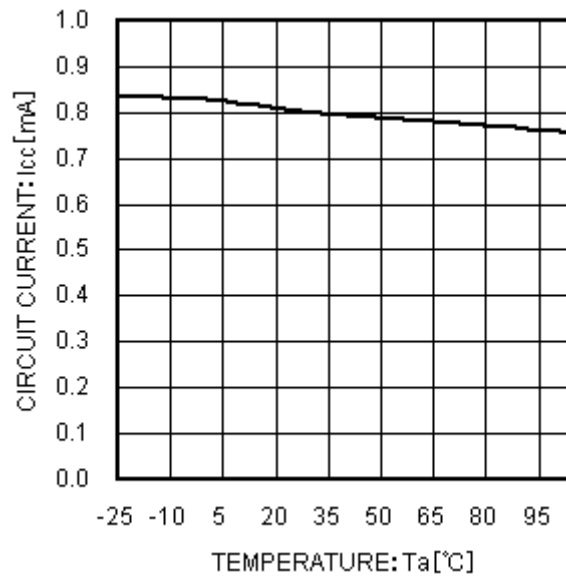
Fig.26 Circuit Current vs Temperature ( I_o=0 mA)
