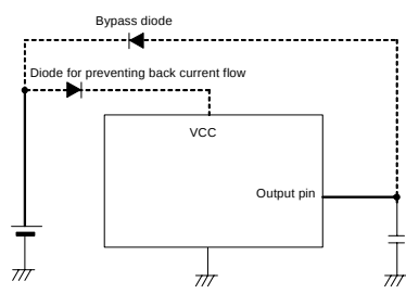
Fig.32 Bypass diode
