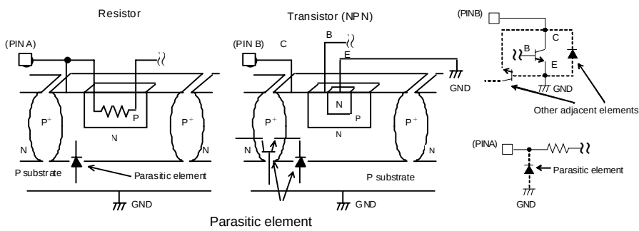
Fig.33 Example of Simple Bipolar IC Architecture
