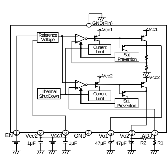
Fig.2 BA30E00WHFP Block Diagram
