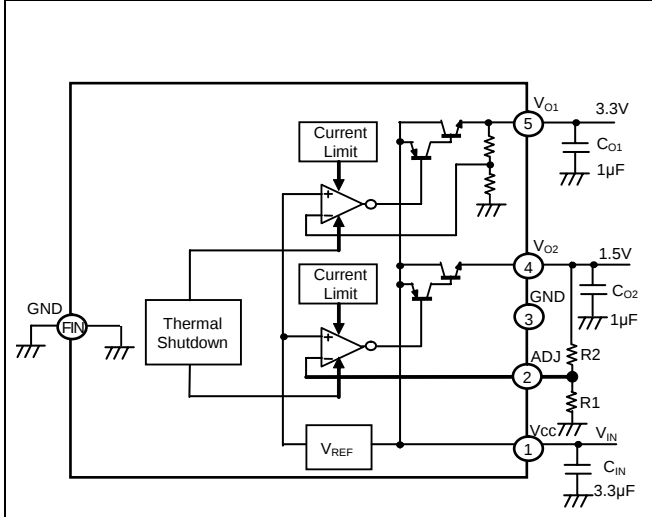
Fig.1 BA3259HFP Block Diagram
