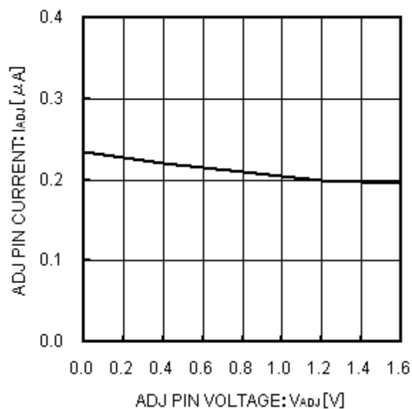
Fig.17 ADJ Pin Source Current
