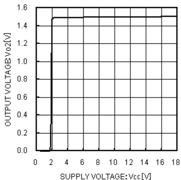
Fig.19 Input Stability (Variable output: 1.8 V)
