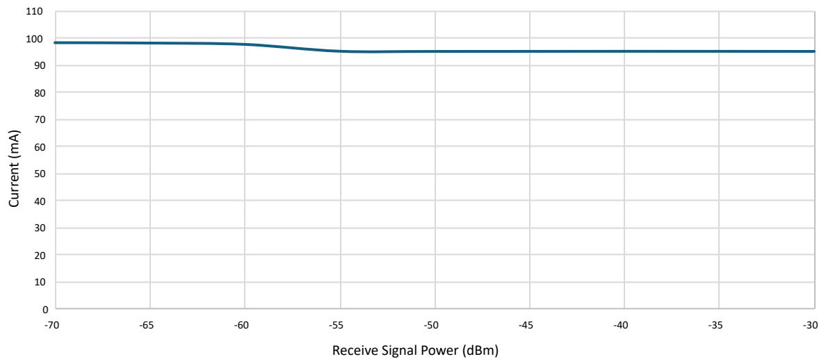
Figure 3-3. Receive Current vs Receive Signal Power, MCS7, Channel 7, 3.3V, 25°C
