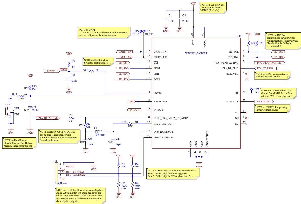
Figure 2-4. WINCS02 Module Basic Connection and Interface Diagram
