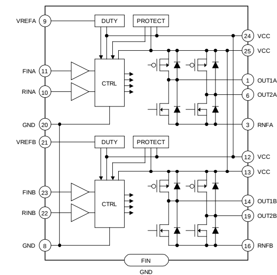
Figure 7. BD6225FP / BD6226FP
