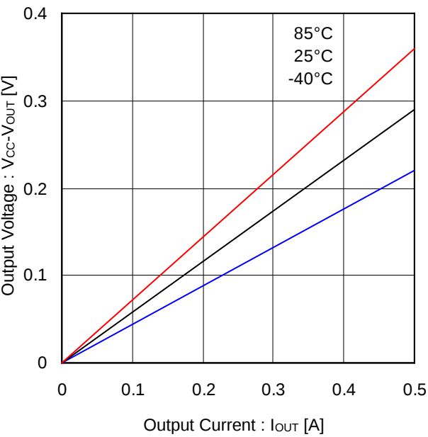
Figure 23. Output High Voltage vs Output Current (BD6222)
