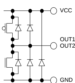
Figure 42. OUT1 / OUT2 (SOP8/HRP7)
