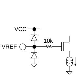
Figure 41. VREF
