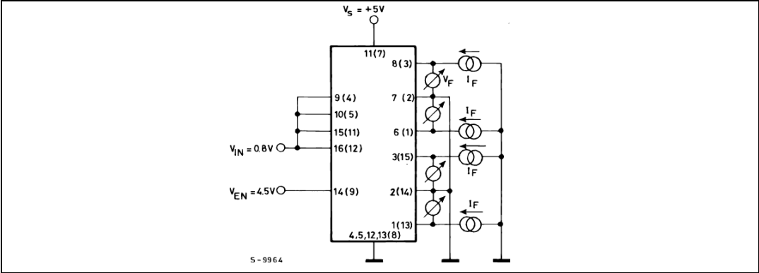
Figure 9. Clamp-diode forward voltage
