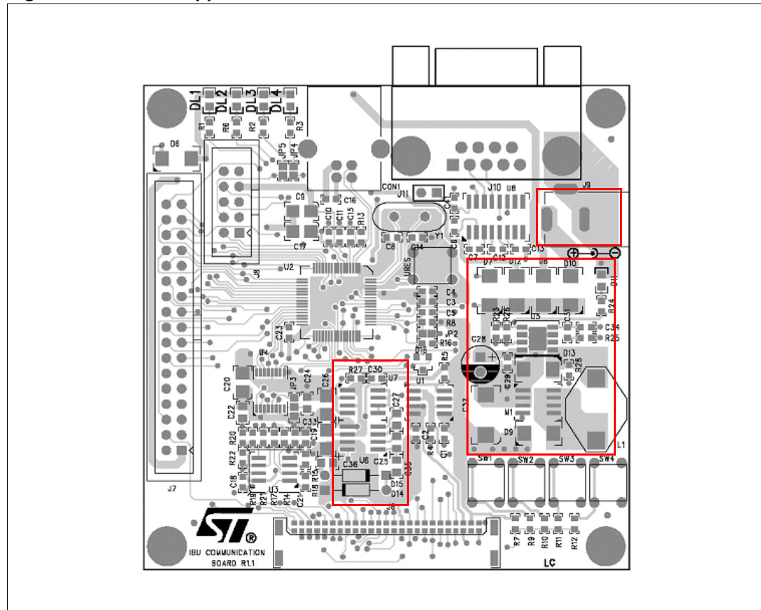
Figure 3. Power supplies PCB area
