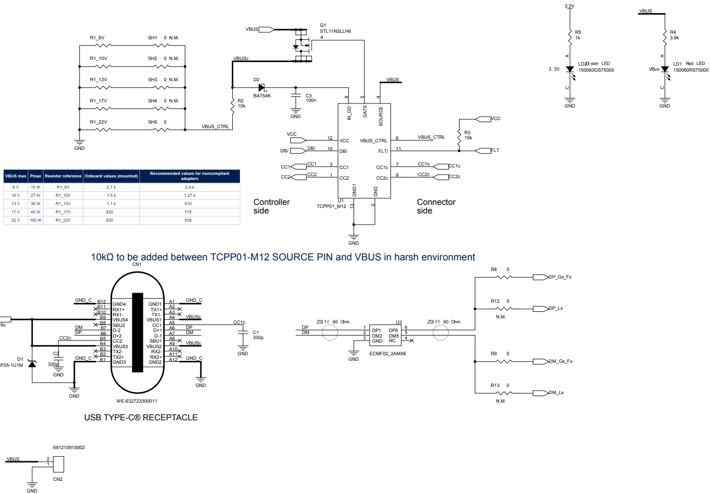
Figure 2. X-NUCLEO-SNK1M1 circuit schematic (2 of 2)
