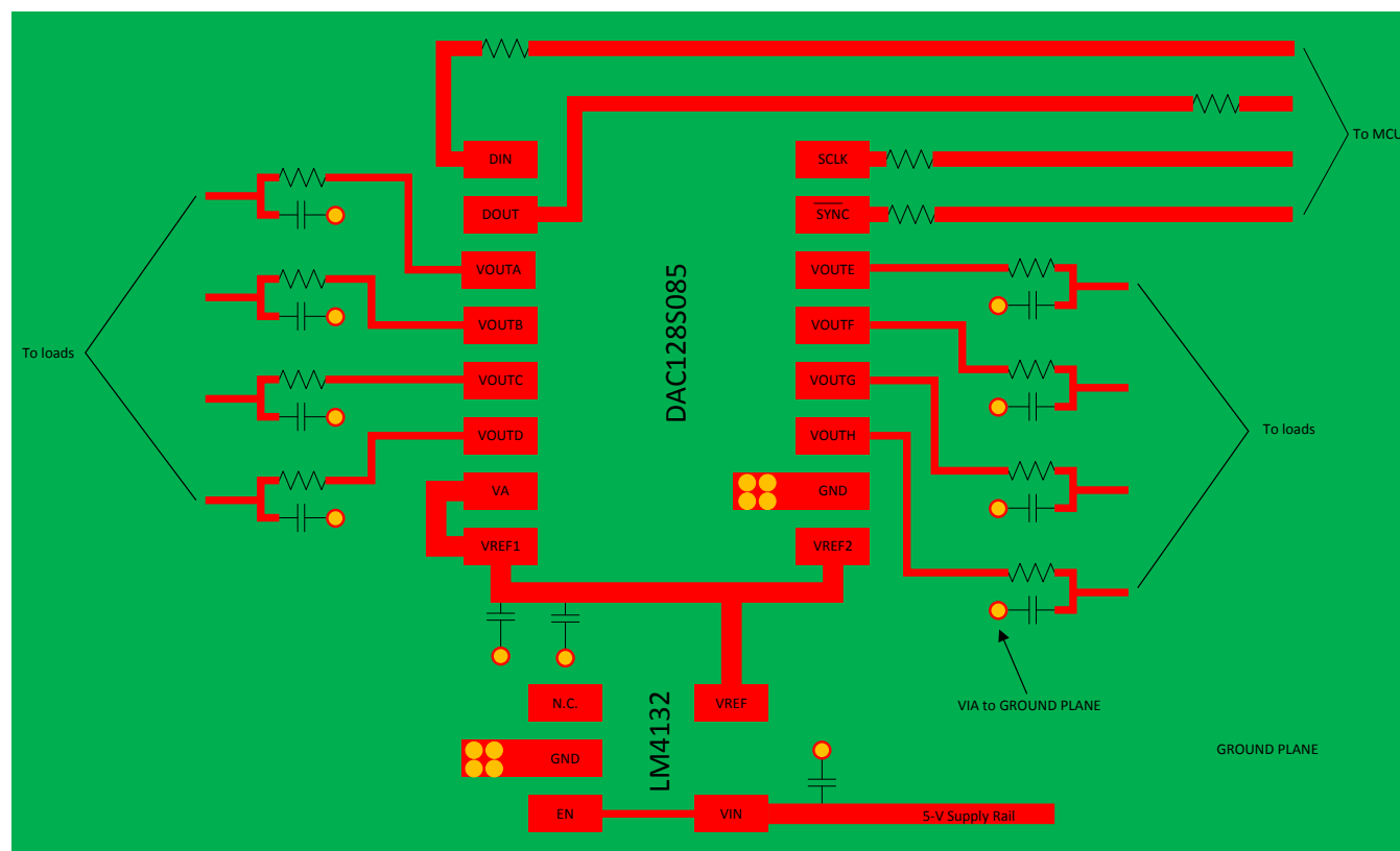
Figure 34. Layout Example
