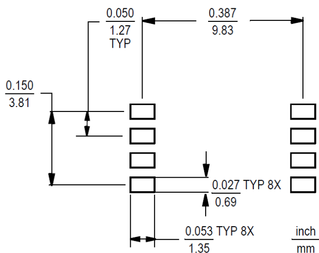
Figure 9. SSOP footprint
