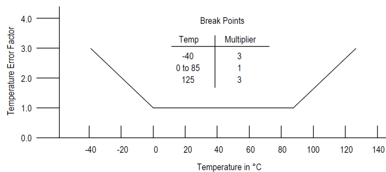
Figure 7. Temperature error band
