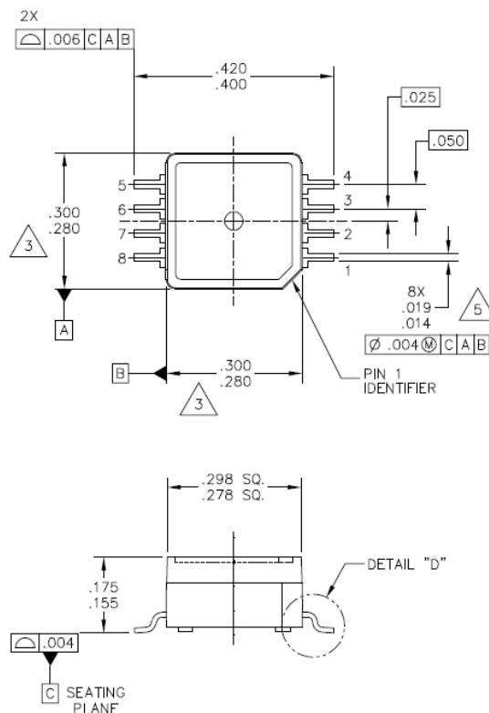
Figure 10. Case 98ARH99066A, super small outline package, surface mount
