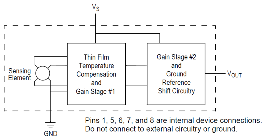
Figure 1. Integrated pressure sensor block diagram
