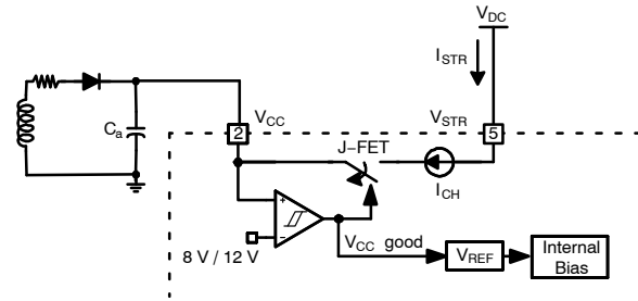
Figure 14. Startup Circuit
