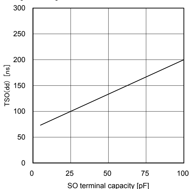
Figure 27. Max of SPI Output Data delay time ( 4.5V \leq V_{DD} \leq 5.5V )
