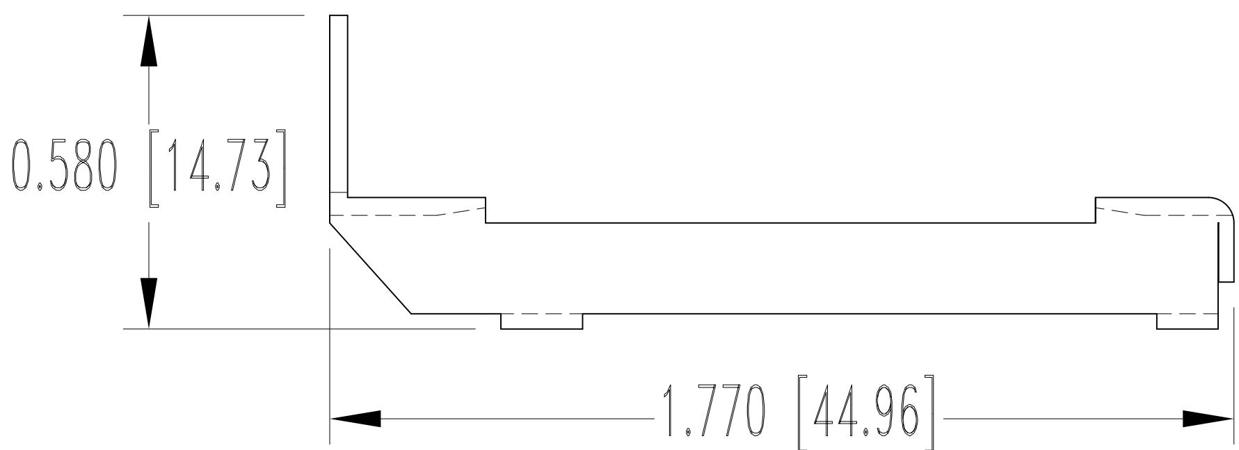
LOCKARM LEVER
