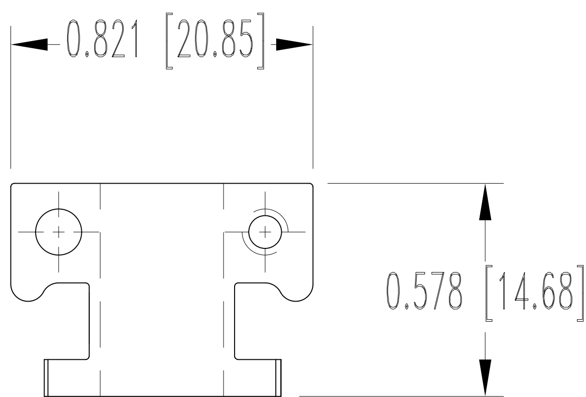
CABLE CLAMP
