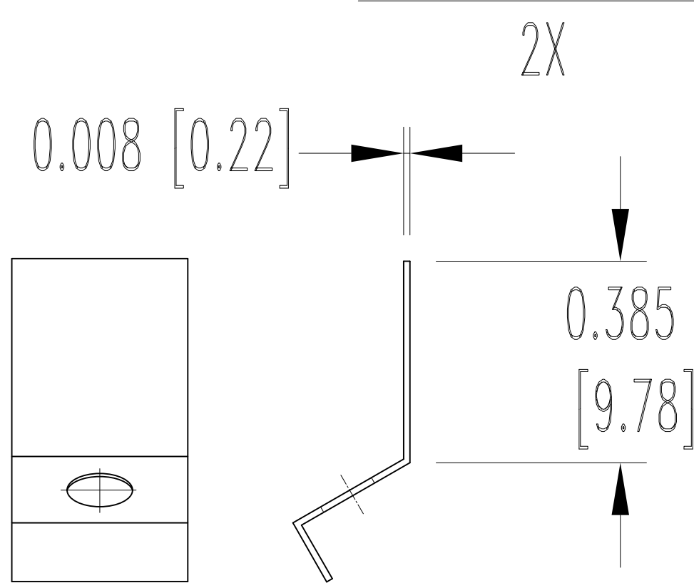
CABLE CLAMP
