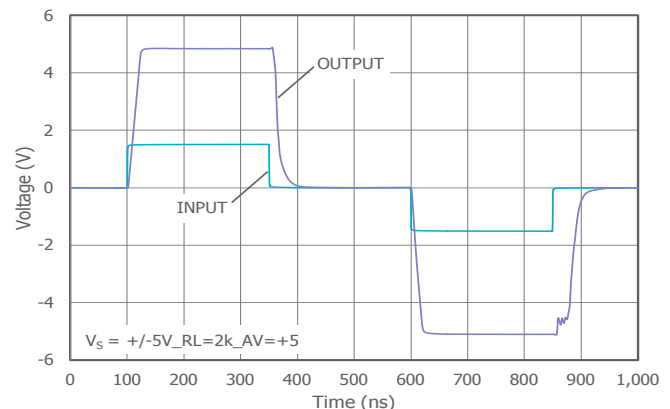
Figure 5: Overdrive Recovery
