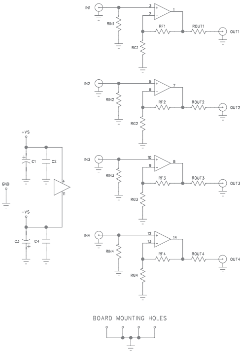
Figure 18. CEB018 Schematic
