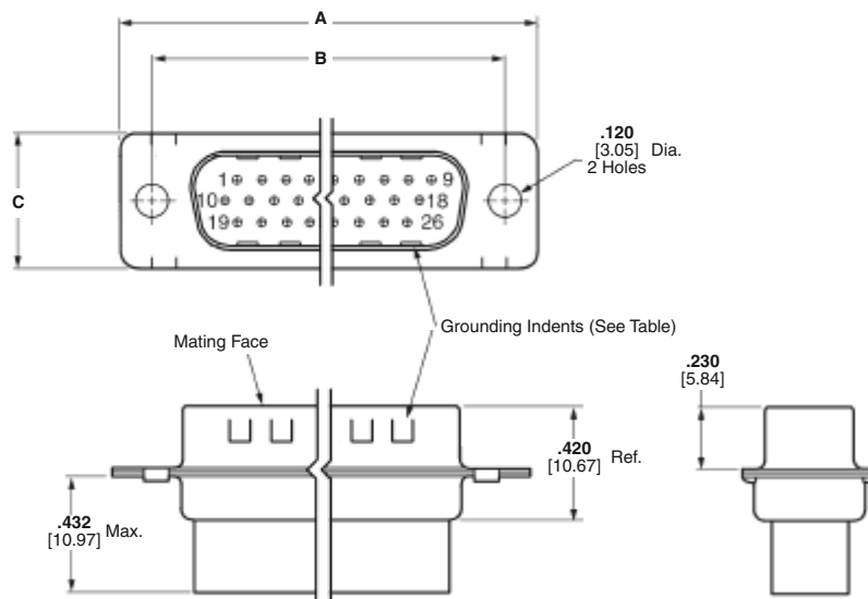
Plug
