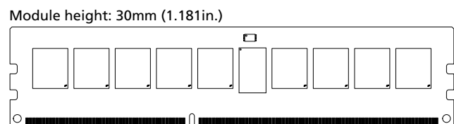
Figure 2: 240-Pin RDIMM (R/C B1)
