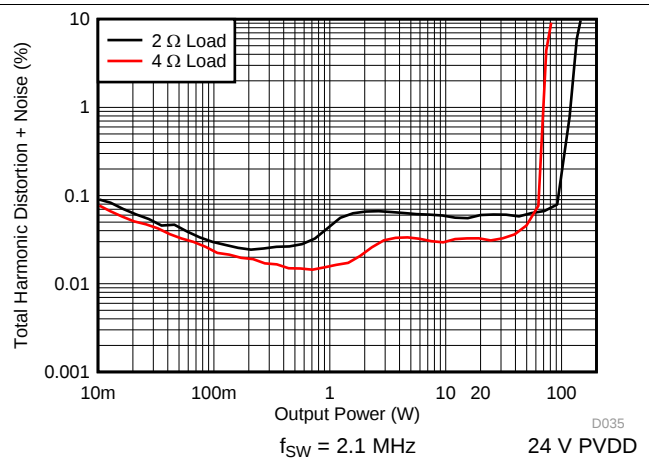
Figure 30. PBTL THD+N vs Power
