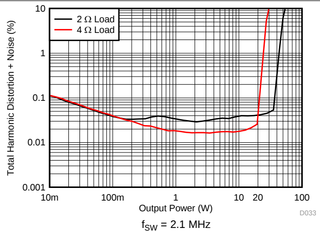
Figure 28. PBTL THD+N vs Power
