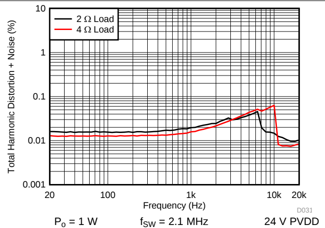
Figure 26. PBTL THD+N vs Frequency
