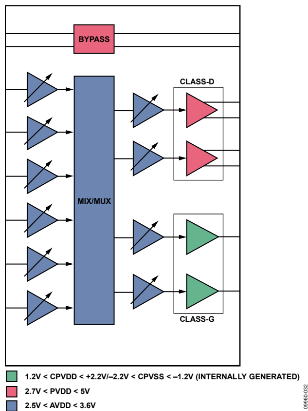
Figure 36. Power Supply Domains
