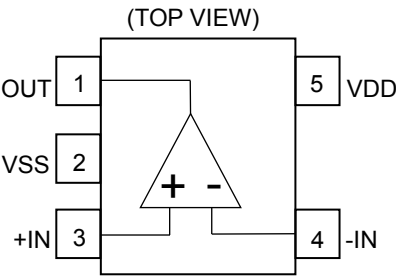
TLR728G-LB (SSOP5)
