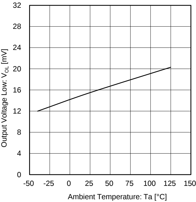
Figure 6. Output Voltage Low vs Ambient Temperature ( V_S = 5\text{ V} , I_L = 1\text{ mA} )
