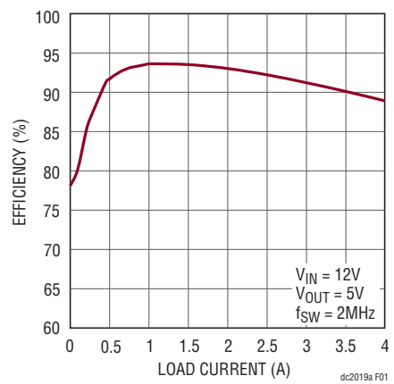
Figure 1. Efficiency vs Load Current (Input from V_{IN} Turret Pin)
