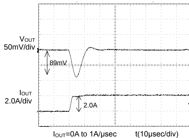
Figure 14. Transient Response (0A to 2.0A) C_{OUT}=47\mu F , C_{FB}=1000pF
