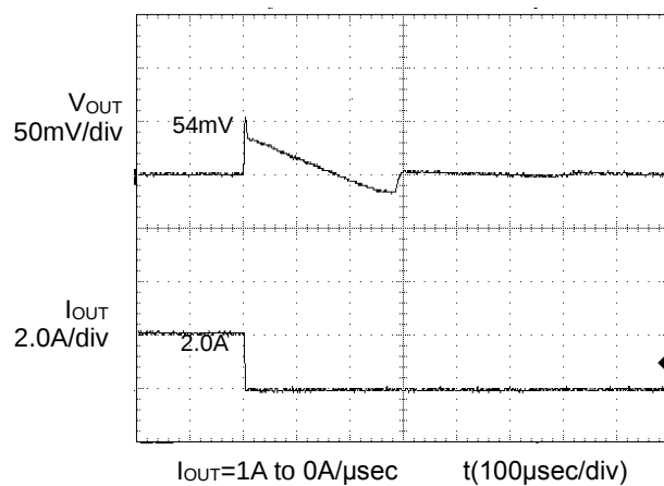
Figure 16. Transient Response (2.0A to 0A) C_{OUT}=100\mu F , C_{FB}=1000pF
