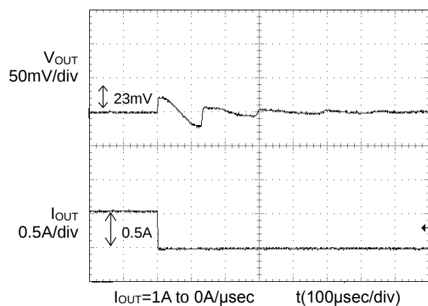
Figure 5. Transient Response (0.5A to 0A) C_{OUT}=47\mu F , C_{FB}=1000pF
