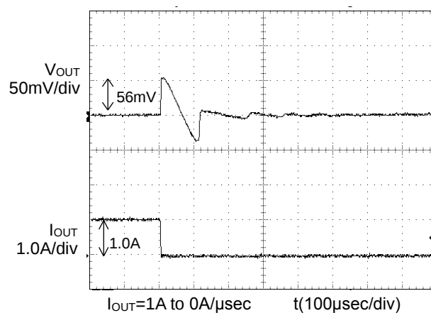
Figure 12. Transient Response (1.0A to 0A) C_{OUT}=22\mu F , C_{FB}=1000pF
