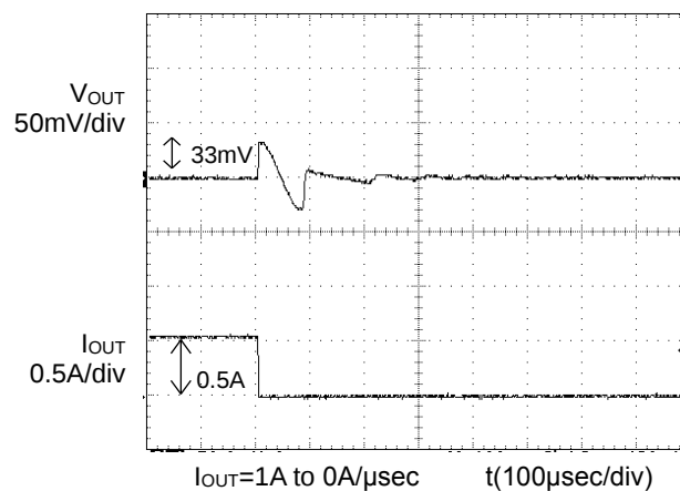
Figure 6. Transient Response (0.5A to 0A) C_{OUT}=22\mu F , C_{FB}=1000pF
