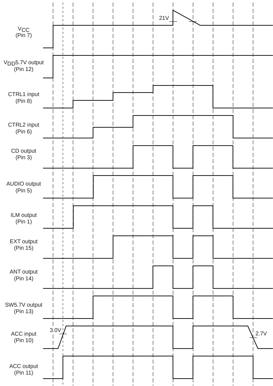
Timing Chart
