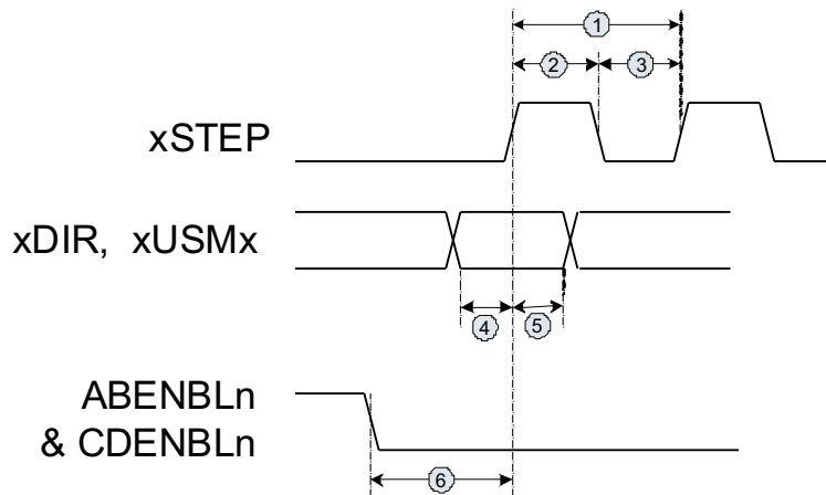
Figure 1. Timing Diagram
