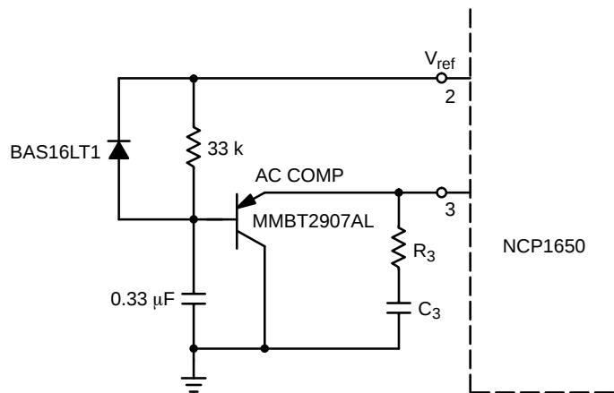
Figure 29. Soft-Start Circuit
