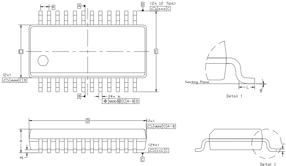
Figure 3. 24-Pin SSOP
