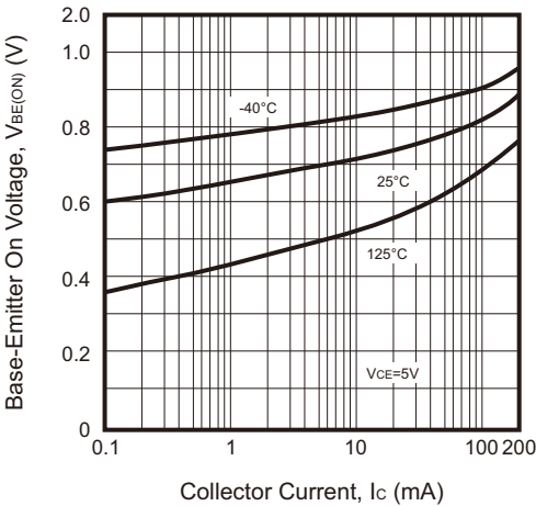
Fig.4 - Base-Emitter On Voltage vs Collector Current
