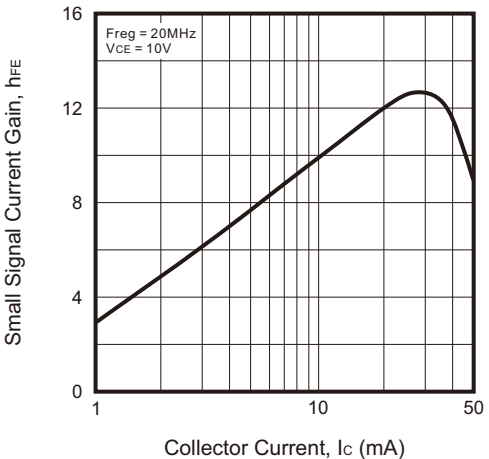
Fig.8 - Small Signal Current Gain vs Collector Current
