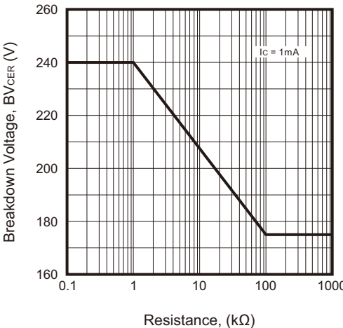
Fig.6 - Collector-Emitter Breakdown Voltage with Resistance Between Emitter-Base
