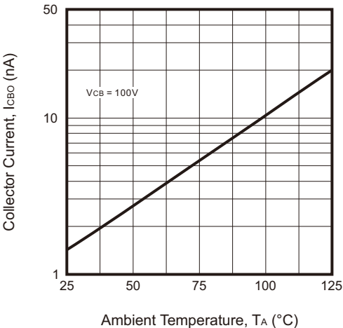
Fig.5 - Collector-Cutoff Current vs Ambient Temperature
