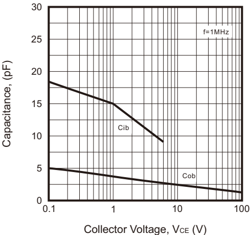
Fig.7 - Input and Output Capacitance vs Reverse Voltage
