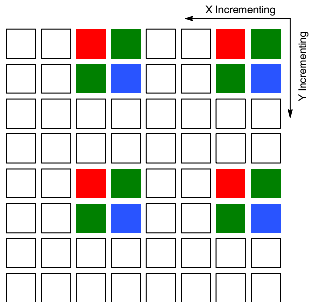
Figure 18. Pixel Readout (Column and Row Skipping)
