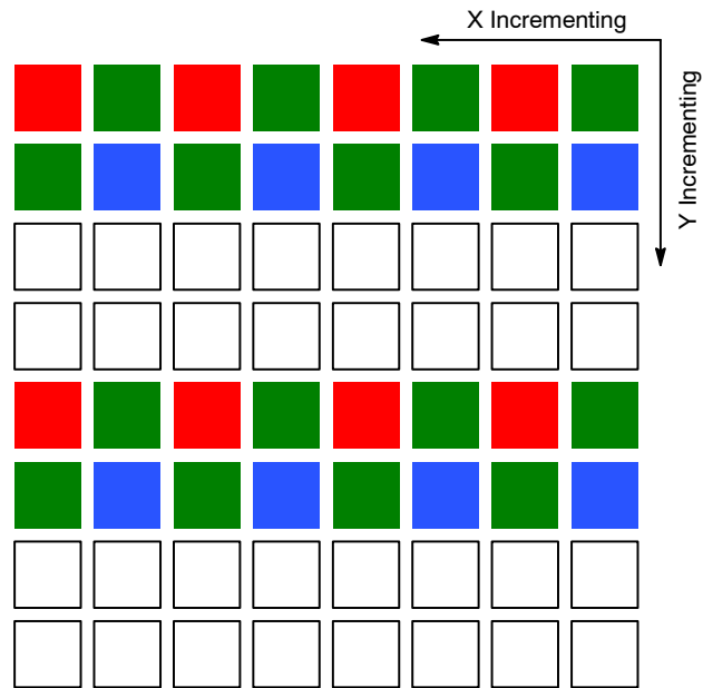
Figure 17. Pixel Readout (Row Skipping)
