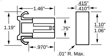
Recommended Panel Mounting Hole (.04" / .078" thick panel)
