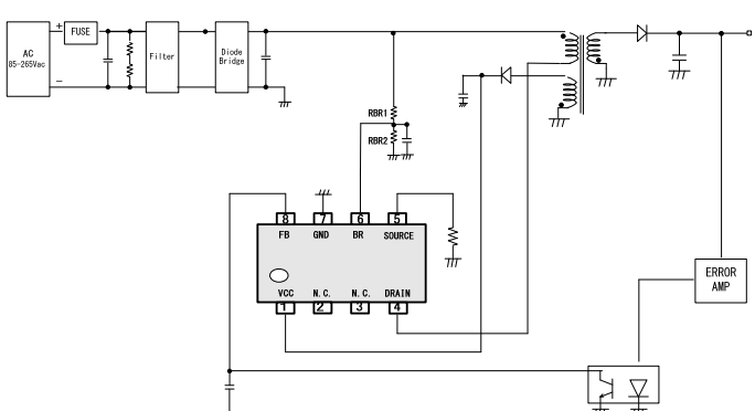
Figure 16(b). DC voltage monitor setting
