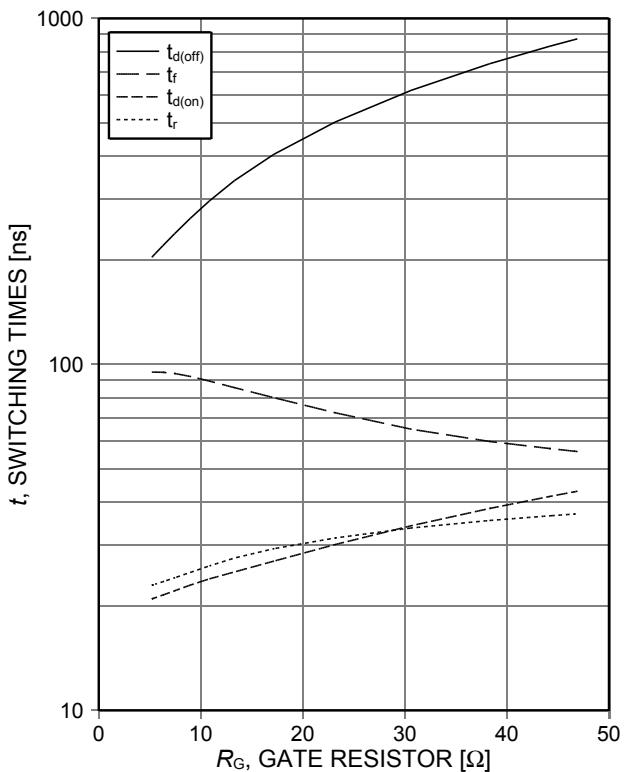
Figure 8. Typical switching times as a function of gate resistor (inductive load, Tj=175°C, VCE=400V, VGE=0/15V, IC=30A, Dynamic test circuit in Figure E)
