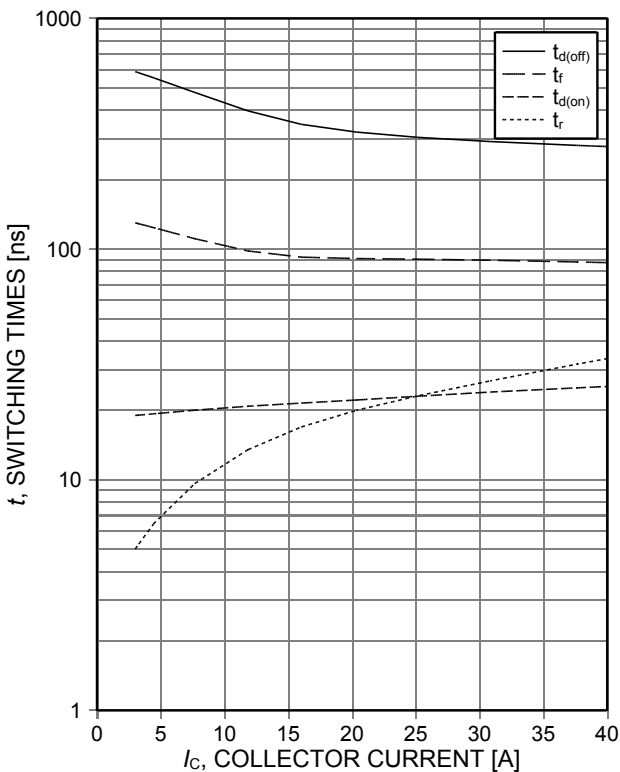
Figure 7. Typical switching times as a function of collector current (inductive load, Tj=175°C, VCE=400V, VGE=0/15V, RG=10Ω, Dynamic test circuit in Figure E)
