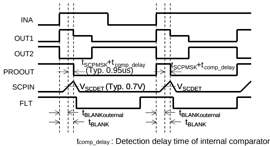
Figure 12. DESAT sequence
