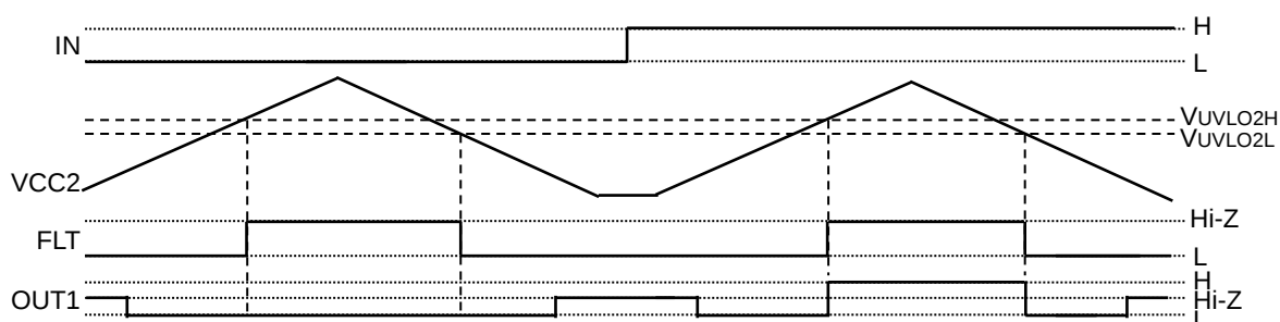
Figure 9. Output-side UVLO Operation Timing Chart
