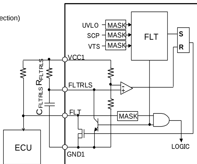
Figure 7. Fault Output Block Diagram
