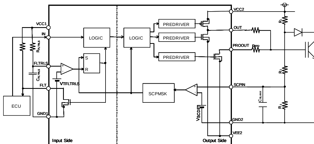
Figure 10. Block Diagram for DESAT
