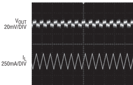
OUT1 Forced Continuous Mode Operation
