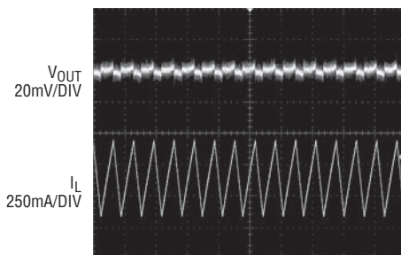
OUT2 Forced Continuous Mode Operation
