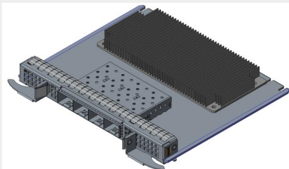
Figure 2 – NIC 3.0 LFF Module (4X SFP version)
