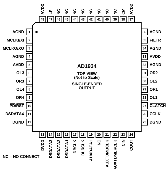
Figure 2. Pin Configuration
