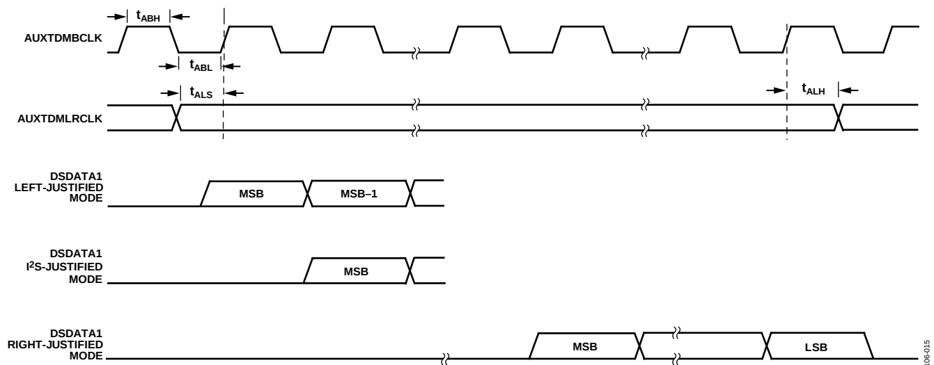
Figure 17. AXTDM Serial Timing
