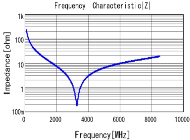
■ GCQ1555C1H6R8DB01 |Z| DC0V, 25degC
