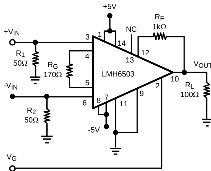
Figure 2. A_{VMAX} = 10V/V
