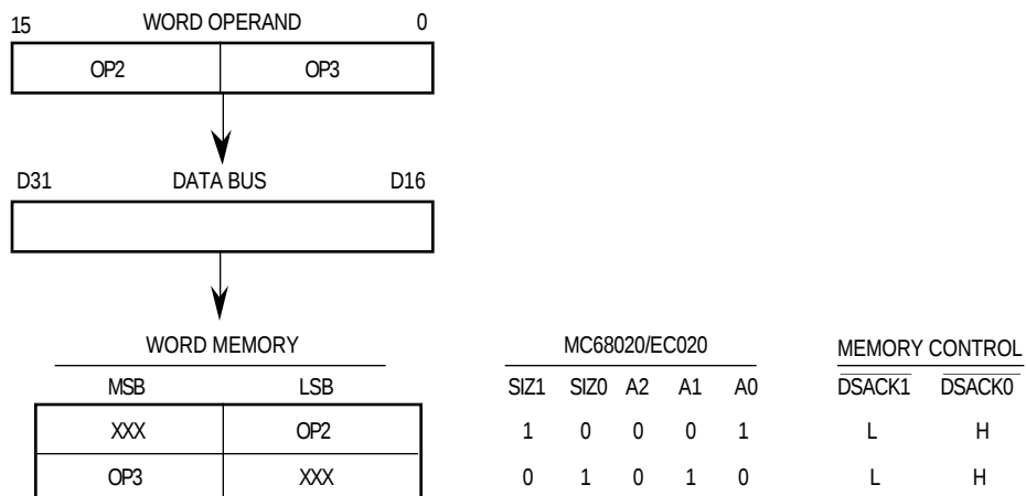
Figure 5-12. Misaligned Word Operand Write to Word Port Example
