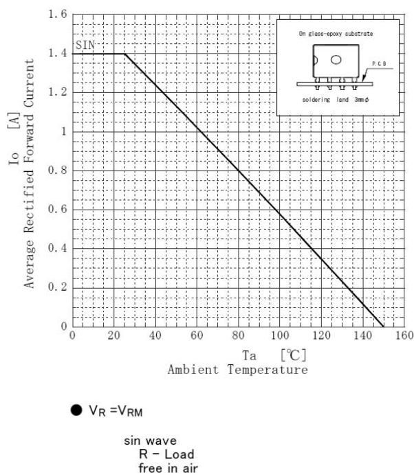
UD8KBA80 Derating Curve
