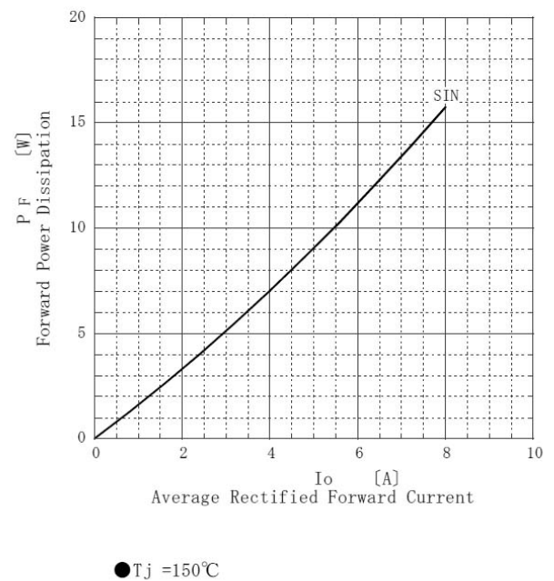
UD8KBA80 Forward Power Dissipation
