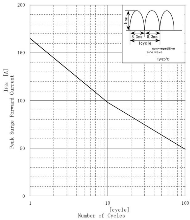
UD8KBA80 Peak Surge Forward Capability
