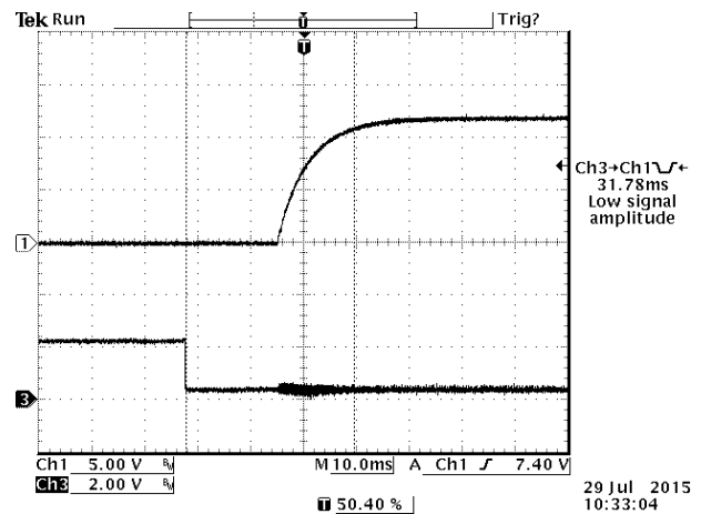
Figure 21. V_{in} = 24\text{ V} , Full Load
