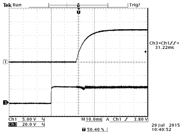
Figure 20. V_{in} = 24\text{ V} , Full Load
