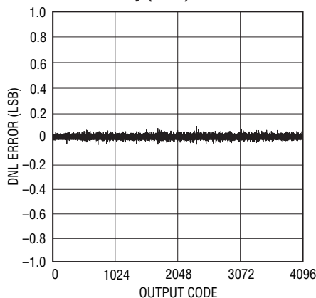
LTC2265-12: Differential Nonlinearity (DNL)
