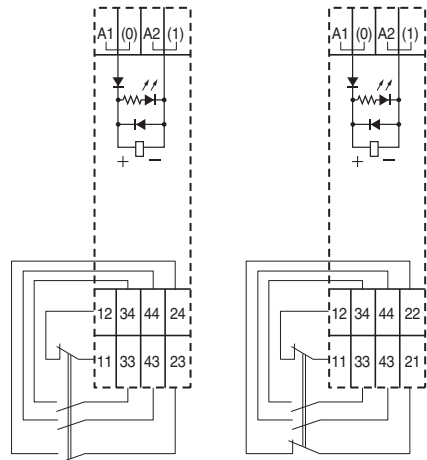
Terminals Arrangement/Internal Connections Diagram (Top View)
