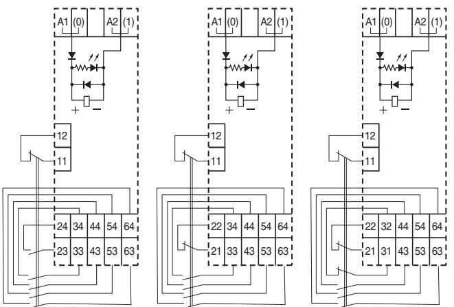
Terminals Arrangement/Internal Connections Diagram (Top View)
