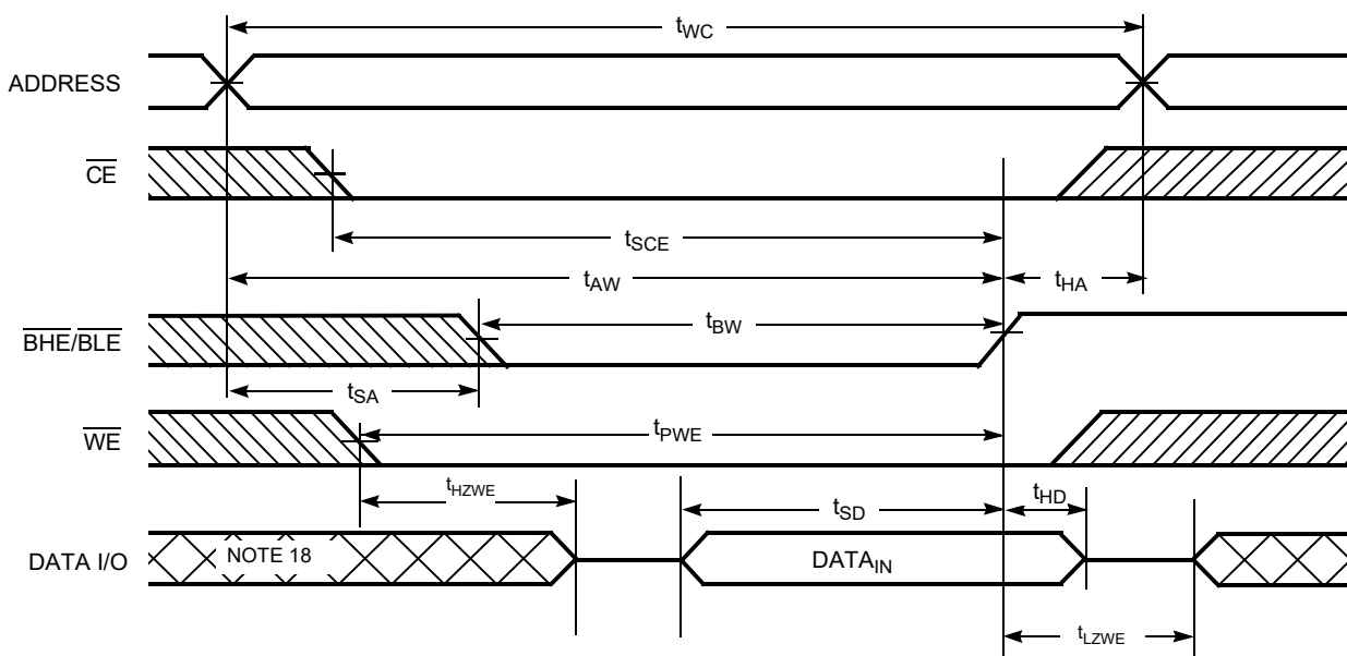
Figure 8. Write Cycle No. 2 ( \overline{\text{BL E}} or \overline{\text{BHE}} Controlled) [15, 16, 17]
