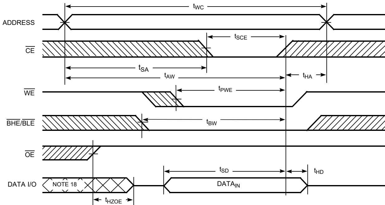
Figure 8. Write Cycle No. 2 ( \overline{\text{BL E}} or \overline{\text{BHE}} Controlled) [15, 16, 17]
