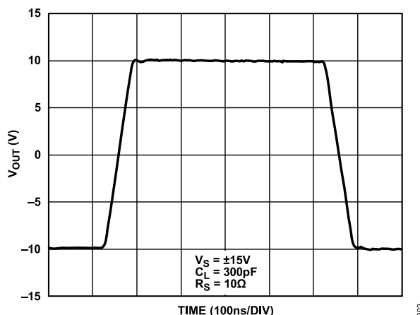
Figure 80. Composite Amplifier Large Signal Pulse Response
