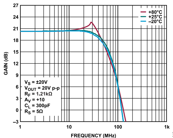
Figure 15. Large Signal Frequency Response vs. Case Temperature, A_V = +10 , V_S = \pm 20\text{ V} , V_{OUT} = 20\text{ V p-p} , R_F = 1.21\text{ k}\Omega , C_L = 300\text{ pF} , R_S = 5\text{ }\Omega
