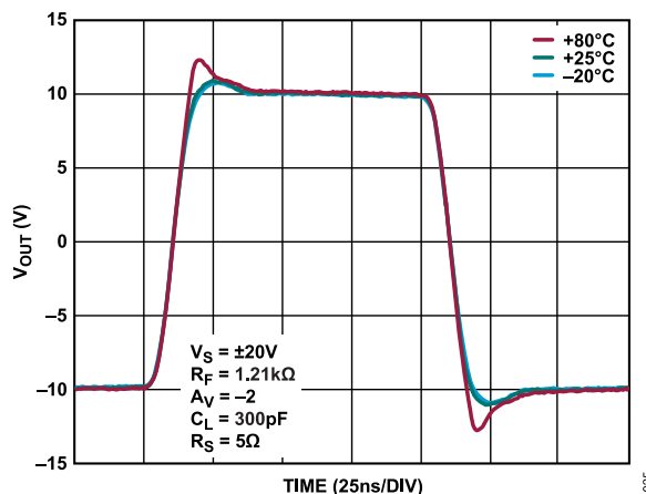
Figure 25. Large Signal Pulse Response vs. Case Temperature, A_V = -2 , V_S = \pm 20\text{ V} , V_{OUT} = 20\text{ V p-p} , R_F = 1.21\text{ k}\Omega , C_L = 300\text{ pF} , R_S = 5\text{ }\Omega
