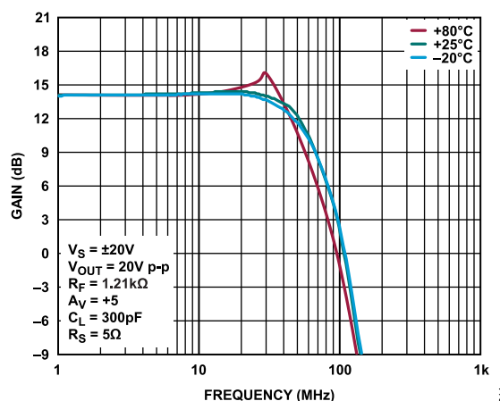
Figure 14. Large Signal Frequency Response vs. Case Temperature, A_V = +5 , V_S = \pm 20\text{ V} , V_{OUT} = 20\text{ V p-p} , R_F = 1.21\text{ k}\Omega , C_L = 300\text{ pF} , R_S = 5\text{ }\Omega
