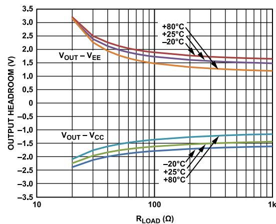
Figure 56. Output Headroom vs. R_{LOAD} Over Case Temperature, V_S = \pm 20\text{ V}
