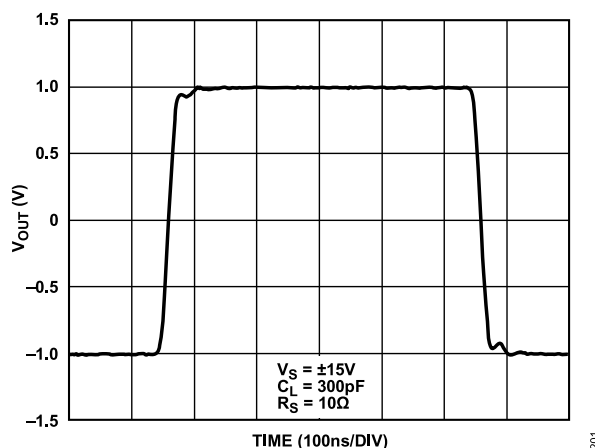
Figure 79. Composite Amplifier Small Signal Pulse Response
