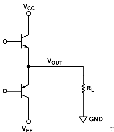
Figure 72. Simplified Output Stage
