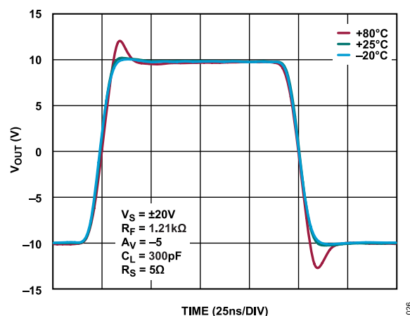
Figure 26. Large Signal Pulse Response vs. Case Temperature, A_V = -5 , V_S = \pm 20\text{ V} , V_{OUT} = 20\text{ V p-p} , R_F = 1.21\text{ k}\Omega , C_L = 300\text{ pF} , R_S = 5\text{ }\Omega
