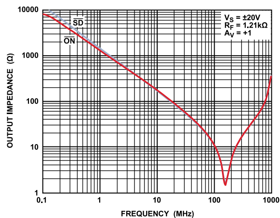
Figure 57. Disabled Closed-Loop Output Impedance vs. Frequency
