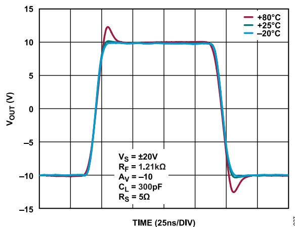
Figure 27. Large Signal Pulse Response vs. Case Temperature, A_V = -10 , V_S = \pm 20\text{ V} , V_{OUT} = 20\text{ V p-p} , R_F = 1.21\text{ k}\Omega , C_L = 300\text{ pF} , R_S = 5\text{ }\Omega
