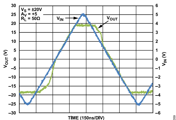
Figure 53. Output Overdrive Recovery, V_S = \pm 20\text{ V} , A_V = +5 , R_L = 50\text{ }\Omega
