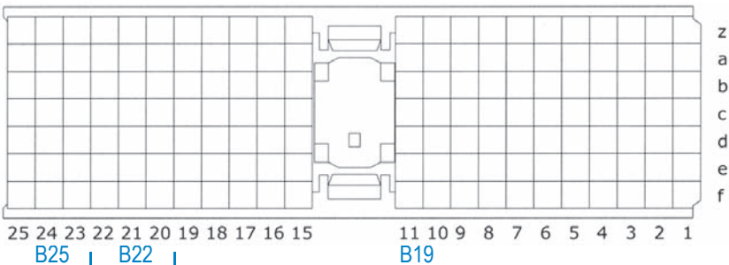
Type-A Connector
