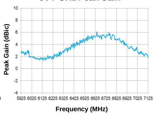
6 / 7 GHz Peak Gain
