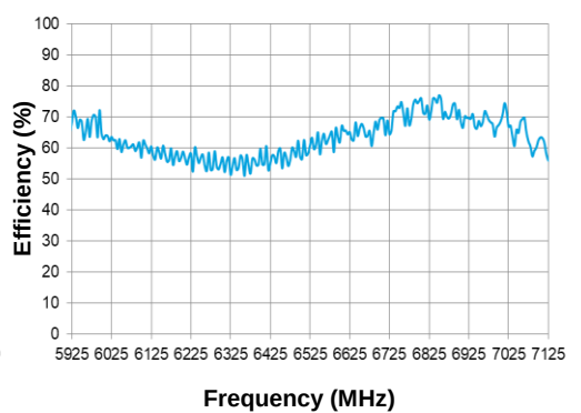
6 / 7 GHz Efficiency
