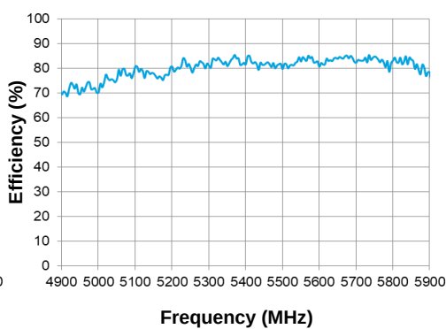
5 GHz Efficiency
