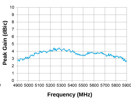
5 GHz Peak Gain
