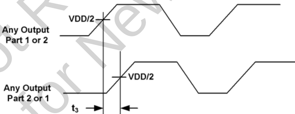
Figure 4. Part-to-Part Skew
