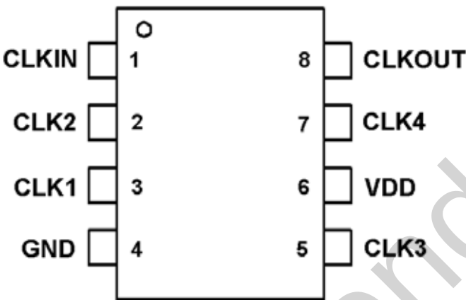
Figure 5. 8-Pin SOIC
