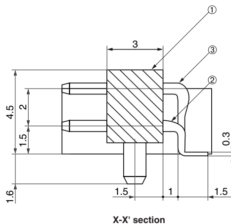
X-X' section
