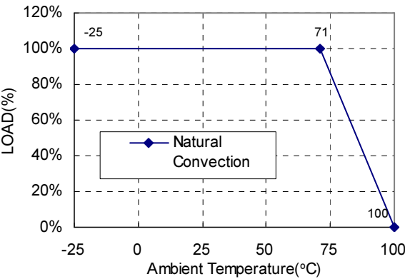
Typical Derating curve for Natural Convection
