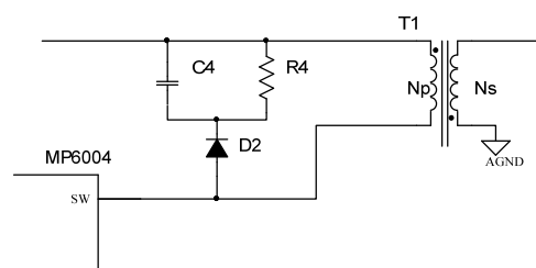
Figure 11: RCD snubber
