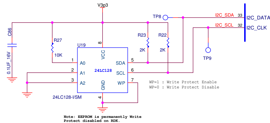
Figure 5-10. I 2 C EEPROM on CY4609 Hardware
