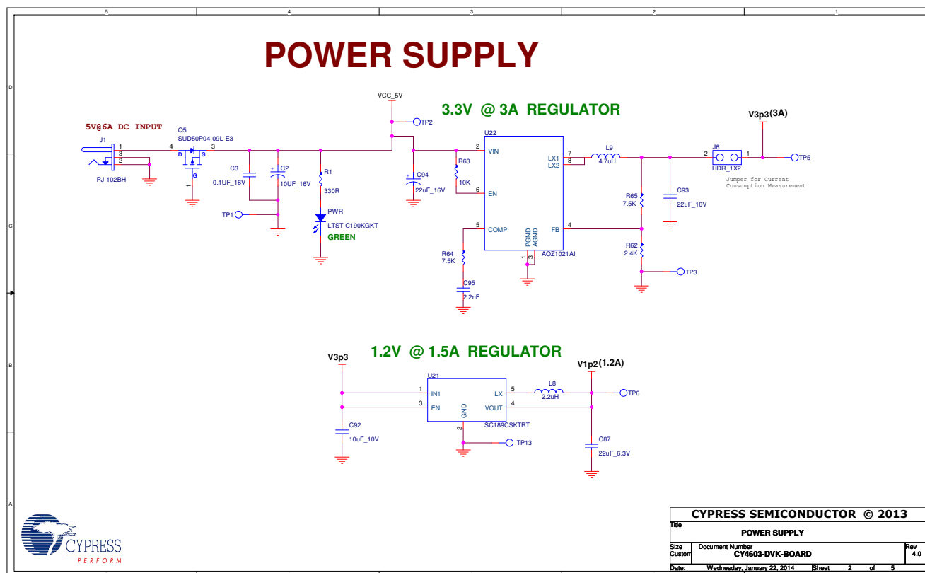
Figure A-4. Voltage Regulators
