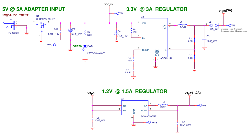
Figure 5-2. Power Regulators for 3.3-V and 1.2-V Power Domains
