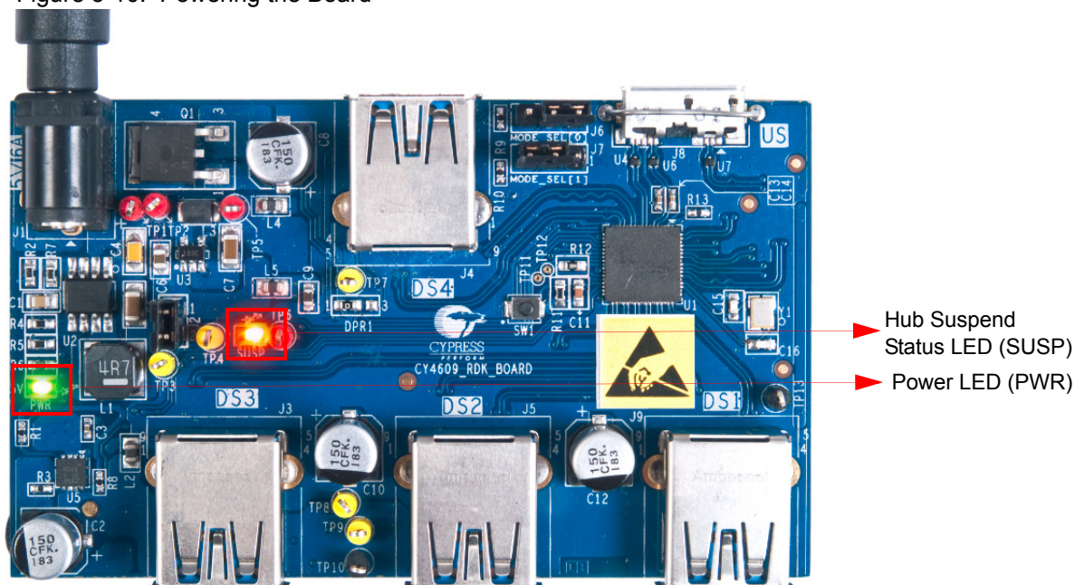
Figure 3-10. Powering the Board
