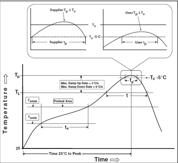
Figure 16 Classification Profile
