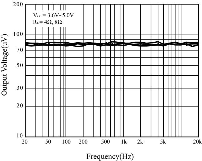
Figure 8 Noise
