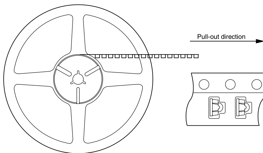
Fig. 13 Product Insertion Direction
